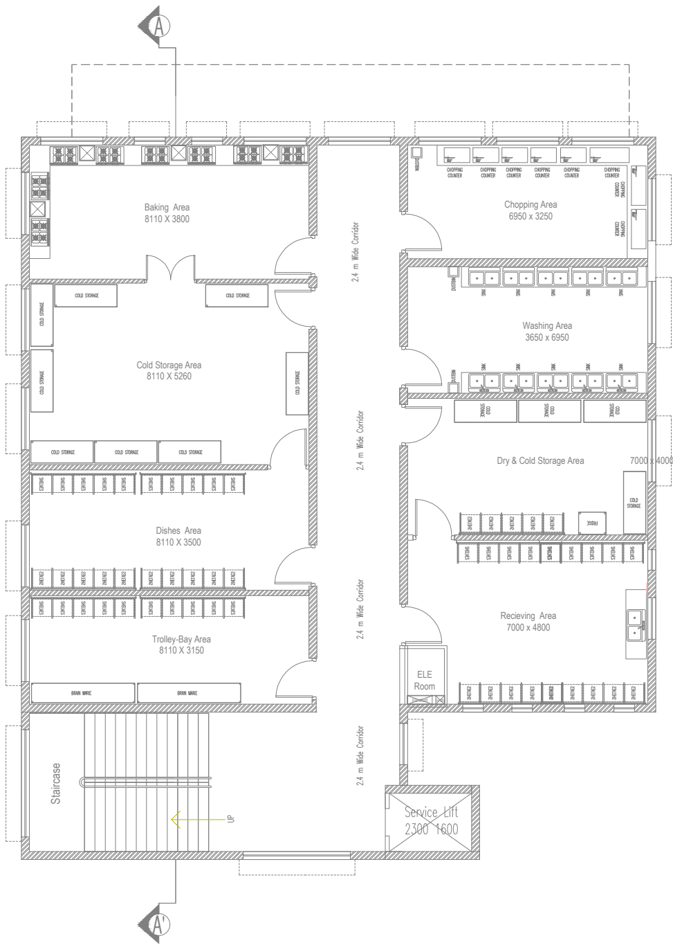
Second Floor SERVICE BLOCK
