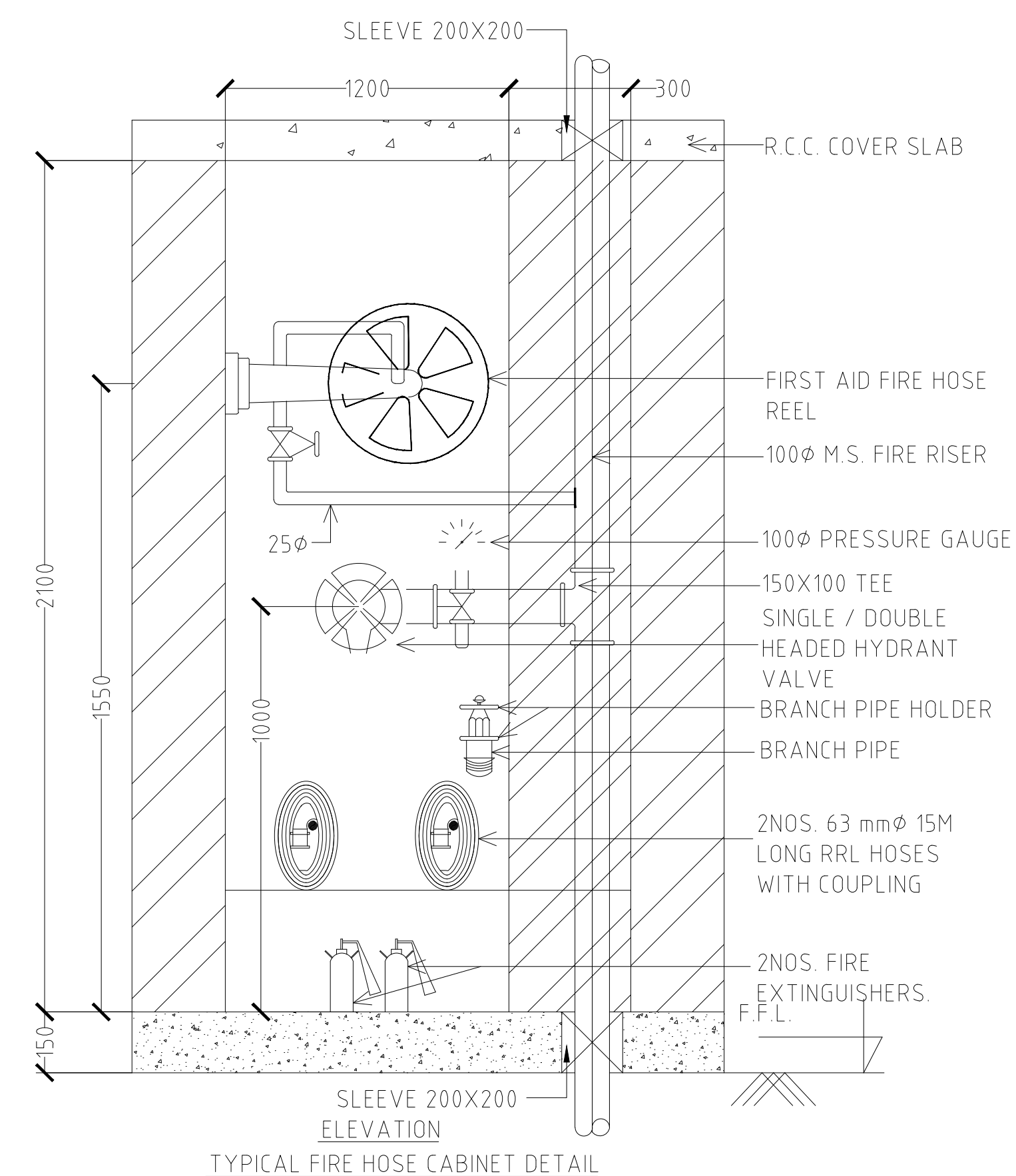
TYPICAL FIRE HOSE CABINET DETAIL
