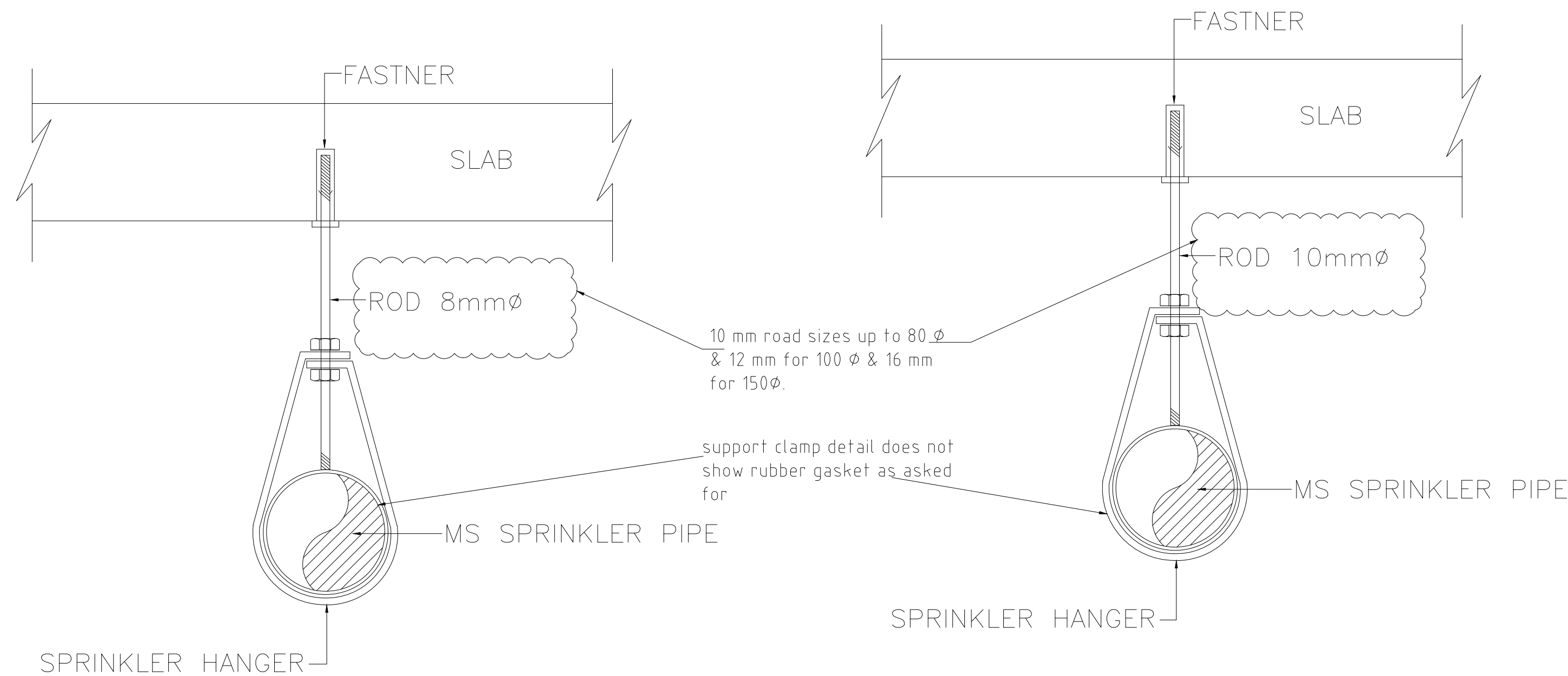
TYPICAL SPRINKLER INSTALLATION DETAIL
