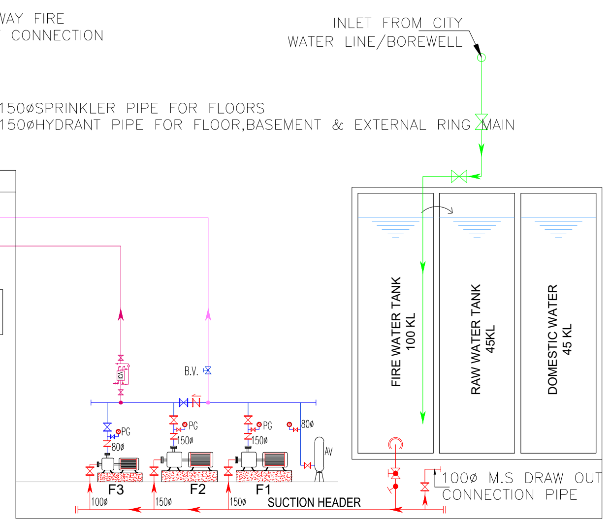
SCHEMATIC DIAGRAM FIRE FIGHTING LAYOUT
