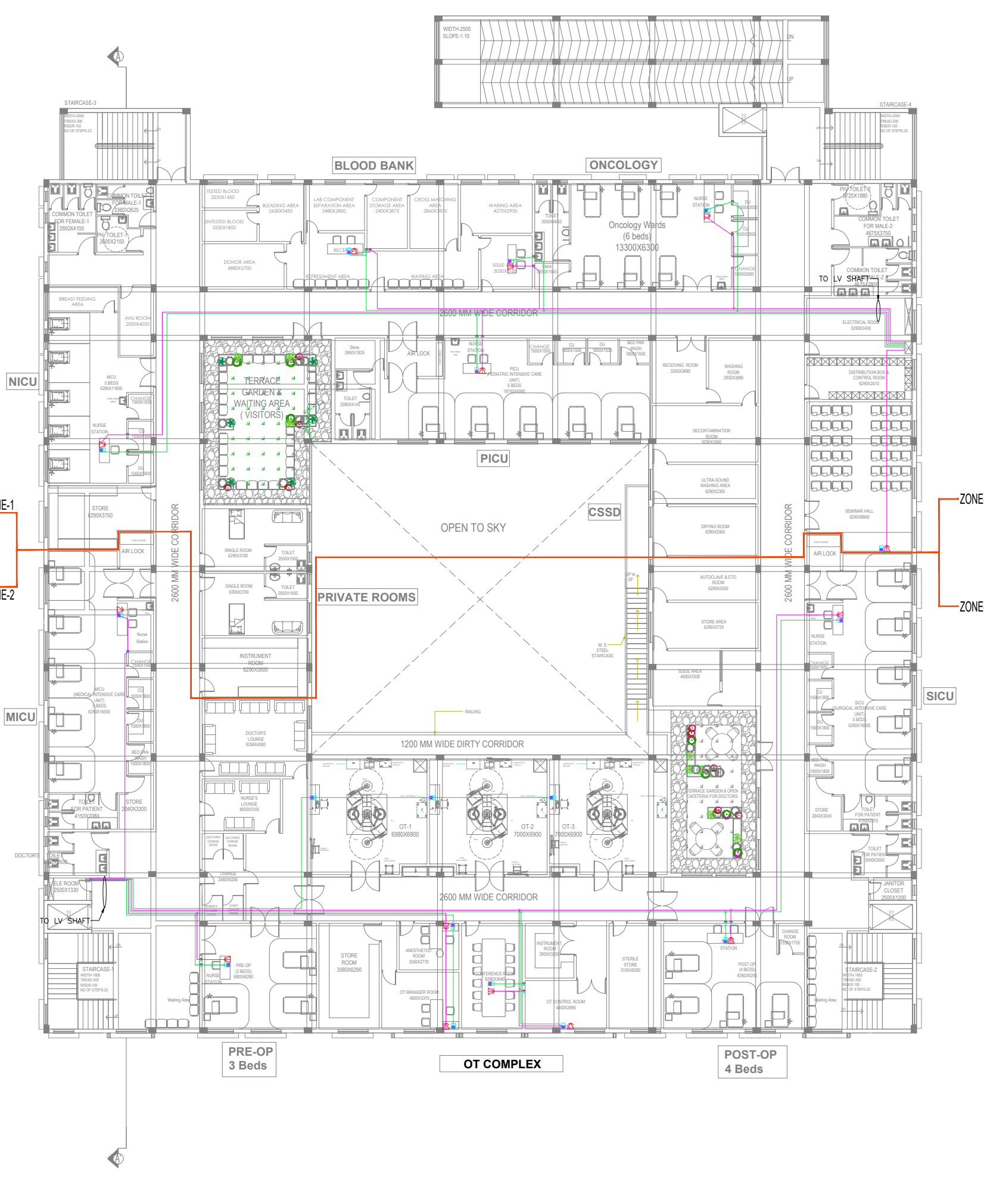
SECOND FLOOR PLAN TOTAL FLOOR AREA=2294.7 SQ.M.
